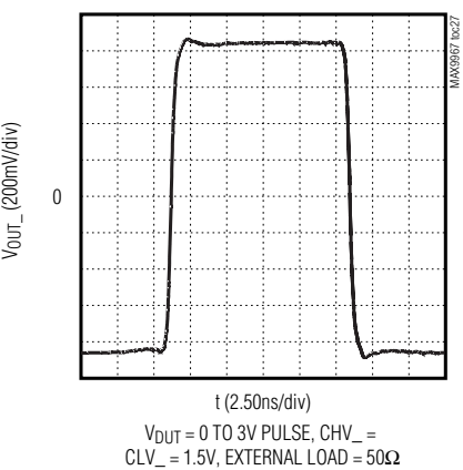
COMPARATOR DIFFERENTIAL OUTPUT RESPONSE (MAX9967_MCCQ)
